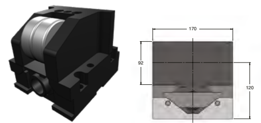
RCP2 150 - Dimensions as per PSA standard
