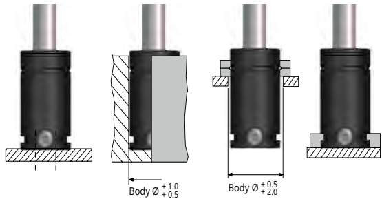
Base mount
