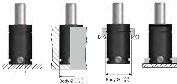
Base mount
