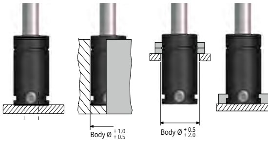
Base mount Drop - in Top mount Foot mount FC, FCS K, FFC
