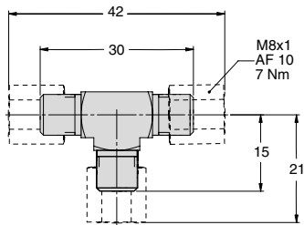
Union Tee Order No. 504592
