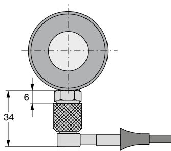
Installation dimensions for hose adapter, with straight and 90° hose
