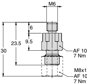
Straight Adapter M6 Order No. 4022057
