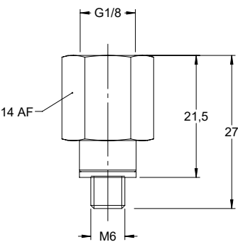
Adapter M6 - G1/8" Order No. 1037553
