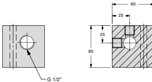
View B-B
