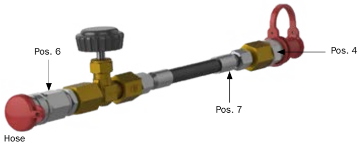
Hose
